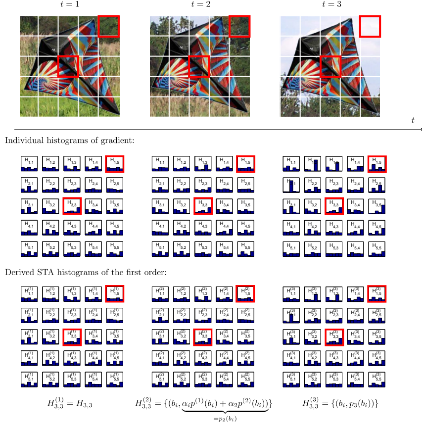
Fig. 1. Constructing the first order STA histograms for a sequence of three frames. Two patches are highlighted in red: a patch which lies in the background and a patch which lies on the object. Notice how the STA histograms of the object patch are constant through time, while the STA histograms of the background patch change.
