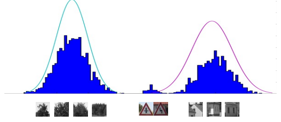
Figure 1: Traffic signs typically do not get represented by a dedicated component of a generative GMM since they are very small with respect to the dimensions of typical images acquired from the driver’s perspective. Therefore, their patches produce large gradients (6) with respect to the closest GMM component, and generate a characteristic contribution to the Fisher vector of the image (8).
